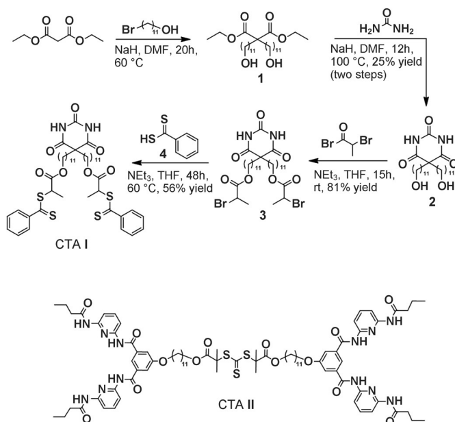
Scheme 1. Synthetic route for the preparation of the CTA I and structure of CTA II.
